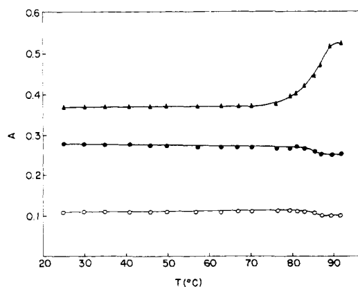
FIGURE 6: Melting profile of poly(br 5 C) · poly(c 7 I) in 0.2 M NaCl-0.01 M sodium cacodylate (pH 7.0). Wavelengths monitored are: 310 nm (○), 300 nm (●), 270 nm (▲).
