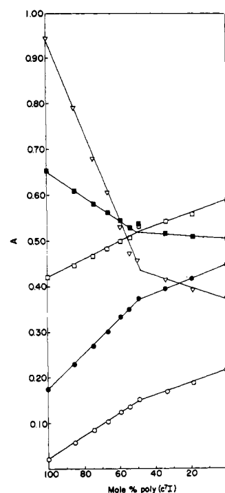
FIGURE 5: Mixing curves (as a function of wavelength) for the interaction of poly(br 5 C) with poly(c 7 I) in 0.2 M NaCl-0.01 M sodium cacodylate (pH 7.0), 22°. Representative wavelengths are as follows: 310 nm (○), 300 nm (●), 290 nm (□), 280 nm (■), 260 nm (▽).
