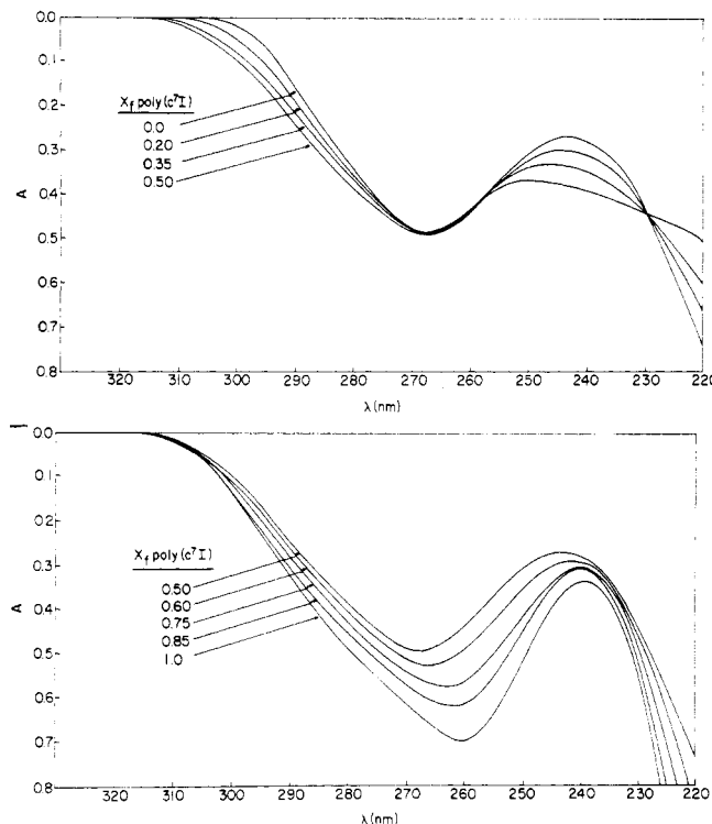
FIGURE 3: Spectra generated from the various solutions used to construct the mixing curve in Figure 2. Upper spectra, 0.0-50 X_f (mole fraction) poly(c 7 I); lower spectra, 0.50-1.00 X_f poly(c 7 I).
