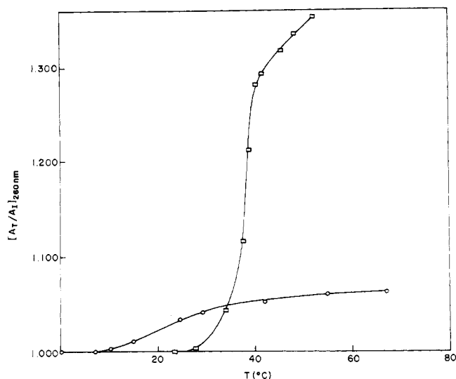
FIGURE 1: Ultraviolet absorbance-temperature profile of poly(c 7 I) (O) and poly(I) (□) both in 1.0 M NaCl-0.01 M sodium cacodylate (pH 7.0). A_T/A_1 is the ratio of absorbance at some given temperature, T , to that at the initial temperature.
