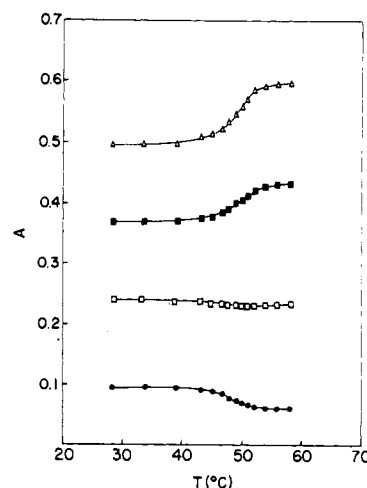
FIGURE 4: Ultraviolet absorbance-temperature profile for poly(c 7 I) · poly(C) (50 mol % poly(c 7 I)) in 0.2 M NaCl-0.01 M sodium cacodylate (pH 7.0). Wavelengths represented are: 300 nm (●), 290 nm (□), 280 nm (■), 267 nm (Δ).
