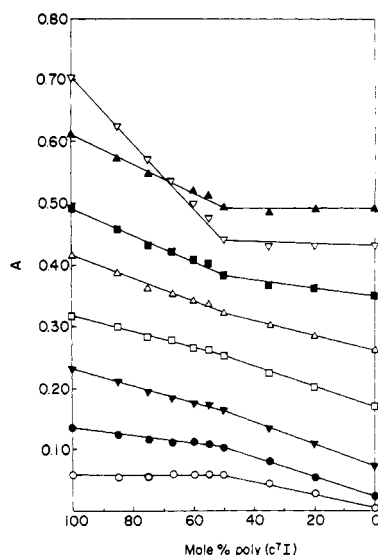
FIGURE 2: Mixing curves as obtained at representative wavelengths for the interaction of poly(C) with poly(c 7 I) in 0.2 M NaCl-0.01 M sodium cacodylate (pH 7.0), 22°. The wavelengths illustrated are: 305 nm (O), 300 nm (●), 295 nm (▼), 290 nm (□), 285 nm (Δ), 280 nm (■), 270 nm (▲), 260 nm (▽).
